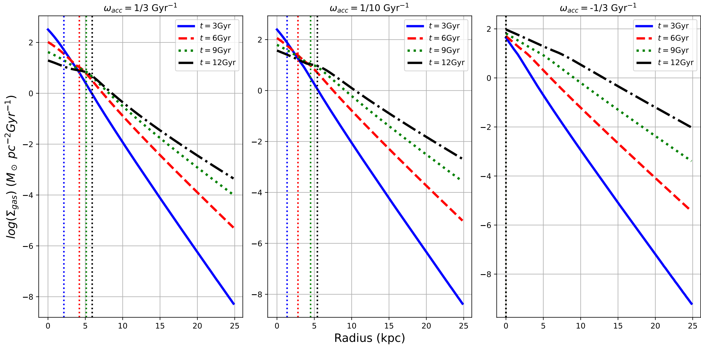
\Sigma_{gas} vs r for different t and t_{acc}
